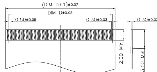
SECTION A-A OPEN TYPE
