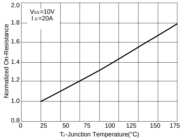
Figure 2: Rdson-Junction Temperature
