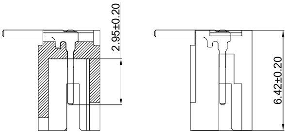
SECTION I-I
