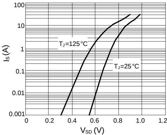
Figure 5: Body-diode characteristics
