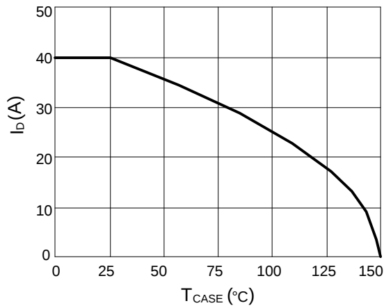
Figure 7: Current de-rating
