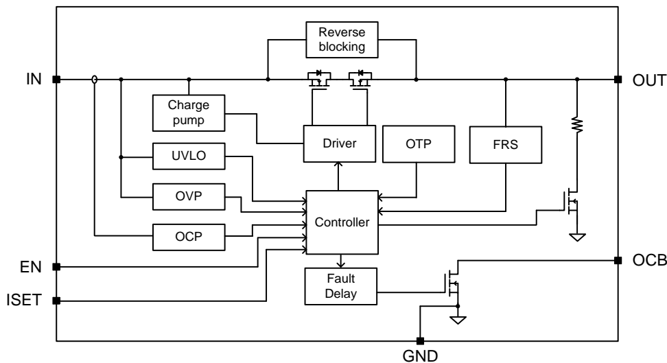
Figure3. Block Diagram
