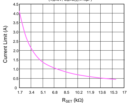
R SET vs. Current Limit (V IN =5V, C IN =C OUT =10μF)
