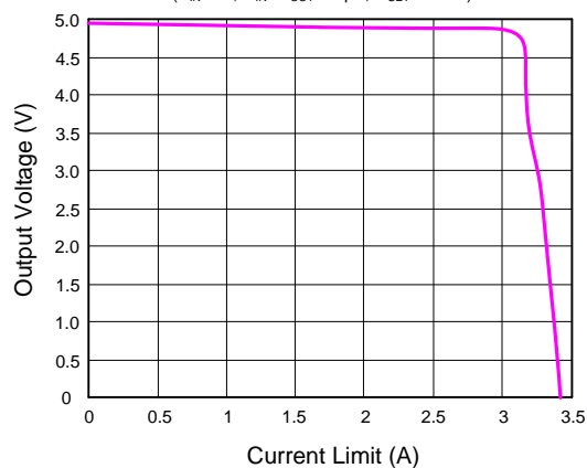
Current Limit vs. Output Voltage (V IN =5V, C IN =C OUT =10μF, R SET =2.2kΩ)
