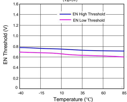
EN Threshold vs. Temperature (V IN =5V)
