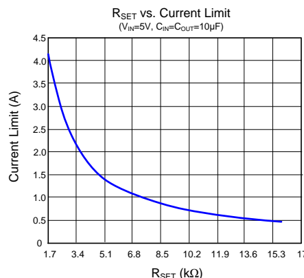
Figure2. R SET vs. Current Limit
