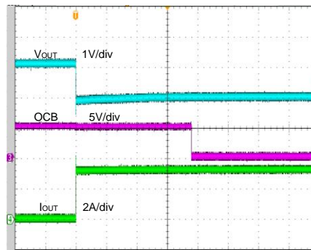
OCB Response During Over Load
