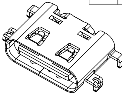
3D VIEW
