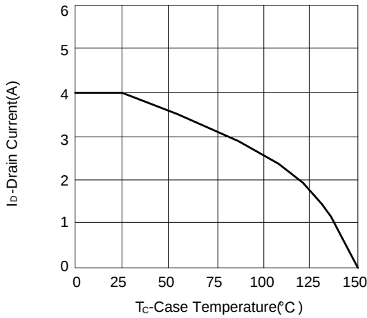
Figure 9: Continuous Drain vs Case Temperature
