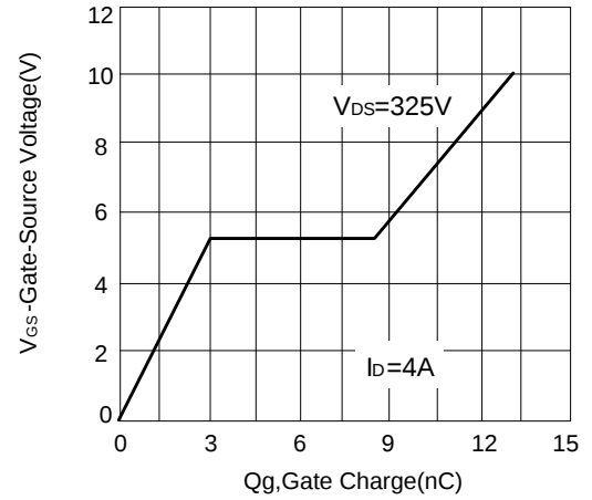
Figure 8: Gate Charge vs Gate to Source Voltage
