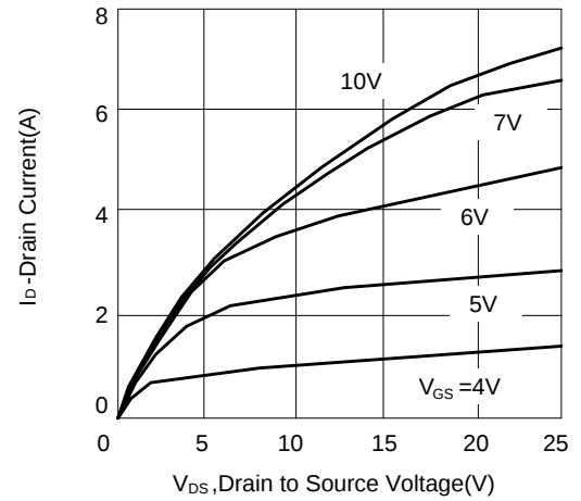
Figure 10: Output Characteristics
