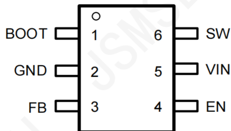
Top View: JSM61410 TSOT23-6L
