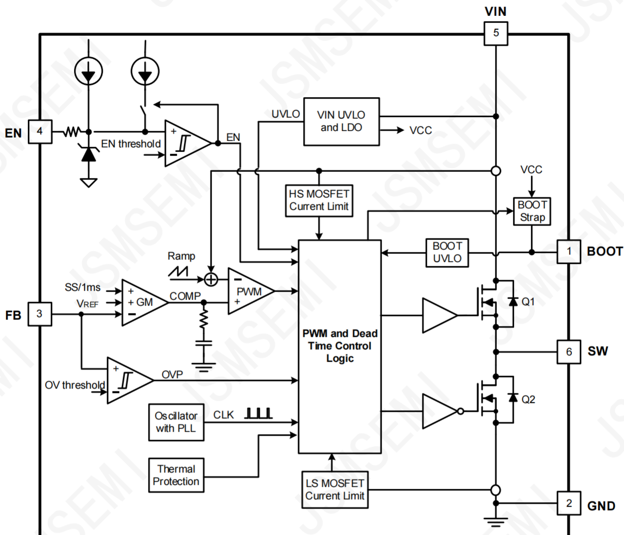
Figure 7. Block Diagram for JSM61410
