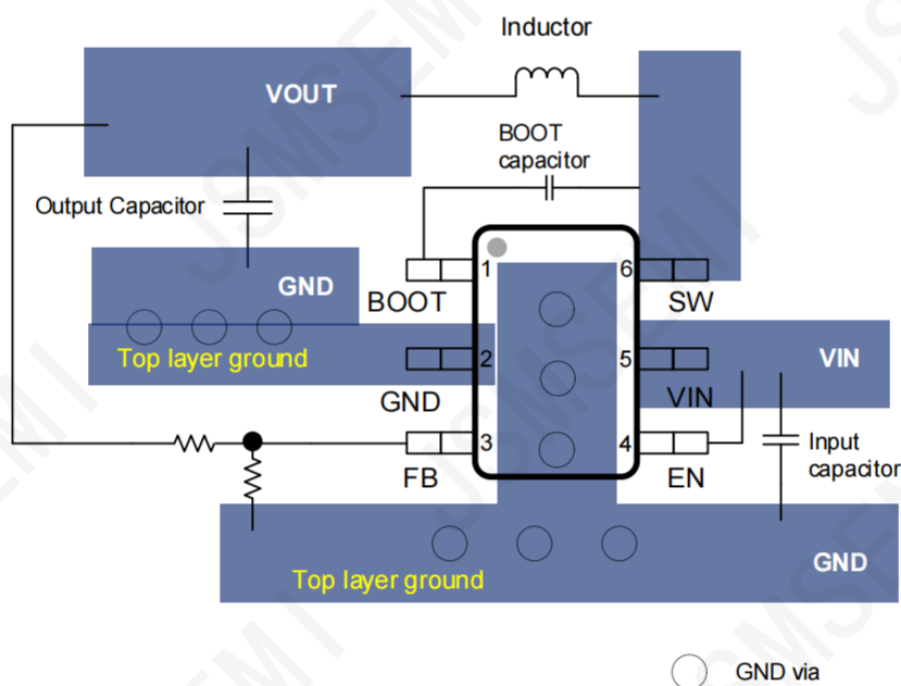
Figure 26. Layout Example
