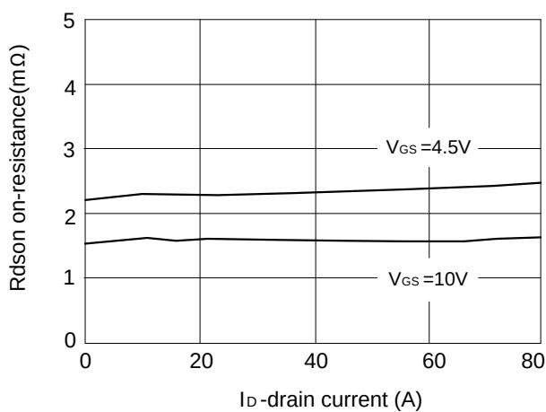
Figure 5 : Rdson-drain current
