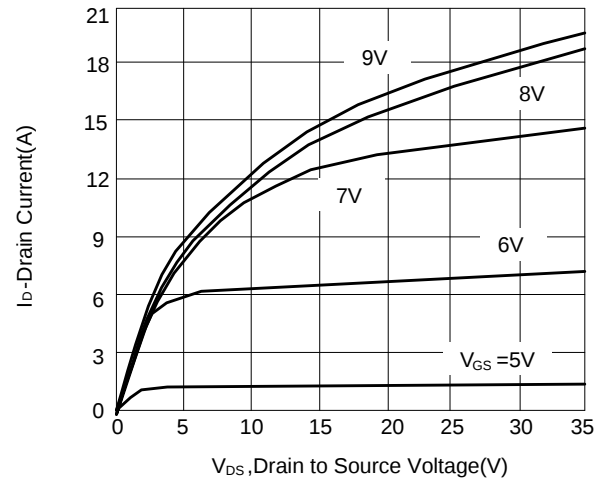
Figure 10: Output Characteristics
