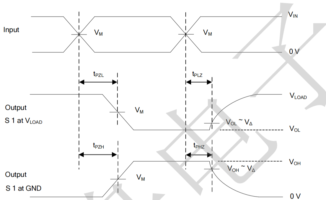
VOLTAGE WAVEFORMS ENABLE AND DISABLE TIMES
