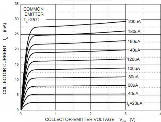
Static Characteristic
