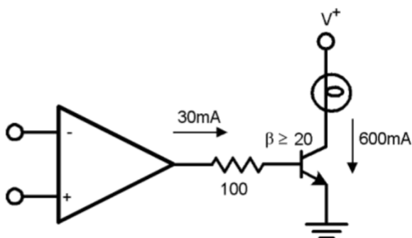
Lamp Driver
