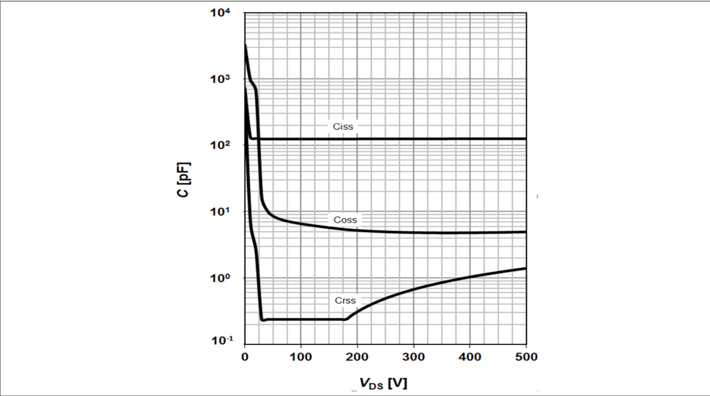
Figure 26 Typical CoolMOS™ capacitances of ICE5BR2280BZ-1; C = f(V_{DS}) , ( V_{GS} = 0 V; f = 250 kHz)
