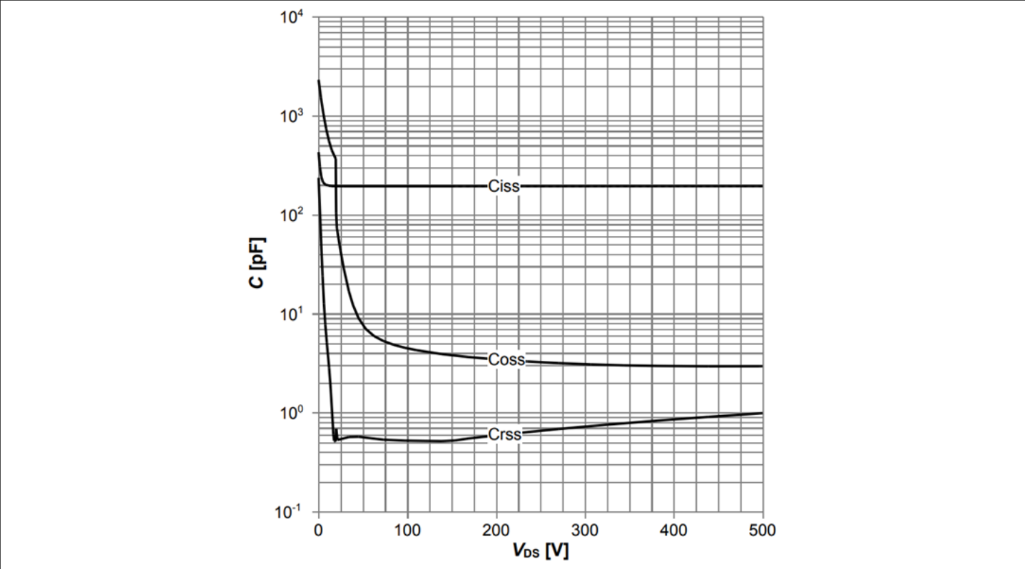
Figure 25 Typical CoolMOS™ capacitances of ICE5xR3995BZ-1; C = f(V_{DS}) , ( V_{GS} = 0 V; f = 250 kHz)
