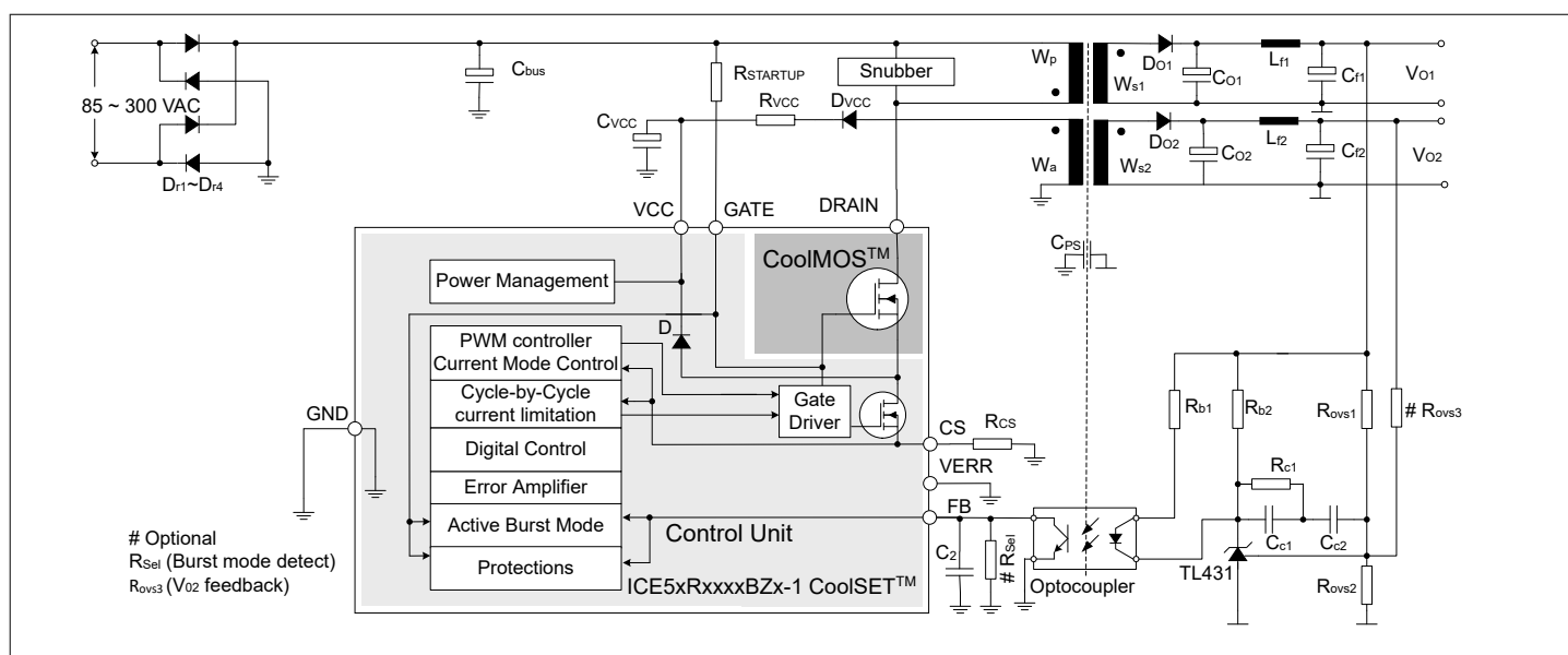
Typical application in an isolated fixed frequency flyback converter using TL431 and an optocoupler
