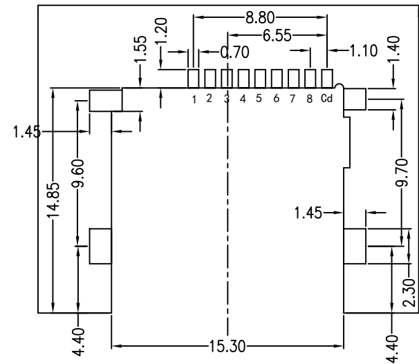
RECOMMENDED P.C.B HOLE LAYOUT COMPONENT SIDE VIEW(TOLERANCE: +/-0.05)
