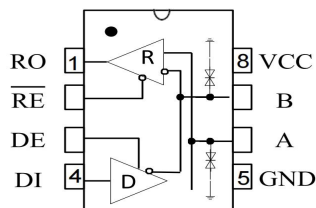
Figure 1 MAX481ESA-TD pin configuration
