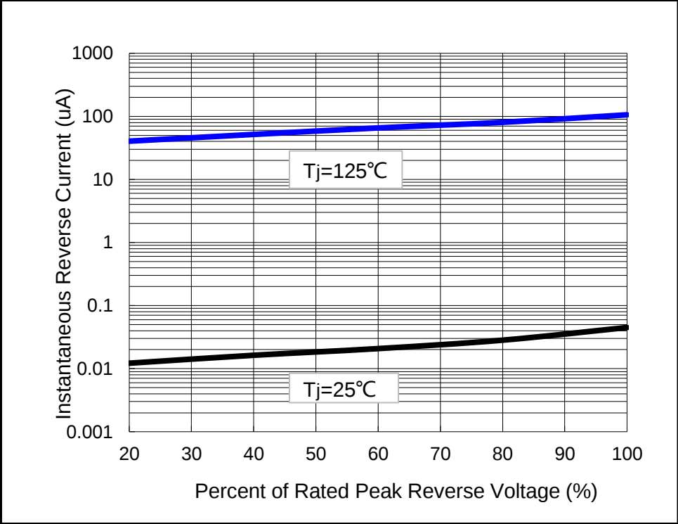
Fig.4 Typical Reverse Characteristics
