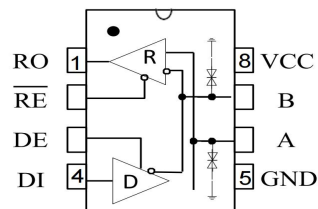
Figure 1 MAX481ECSA-TD pin configuration
