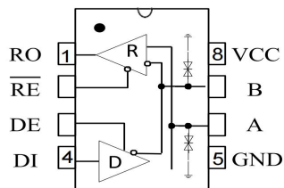
Figure 1 MAX483ESA-TD pin configuration
