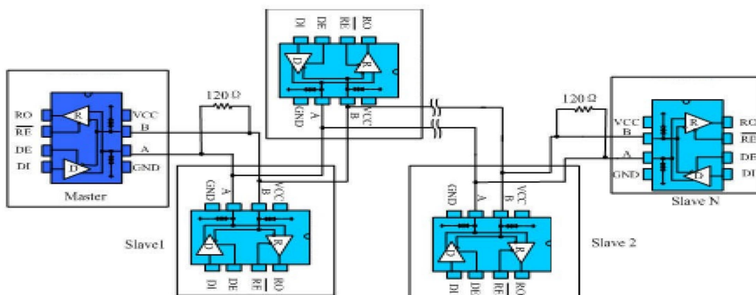
Fig. 10 Hand-in-hand type RS485 half-duplex communication network
