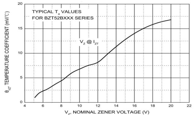
Fig.2 Temperature Coefficients
