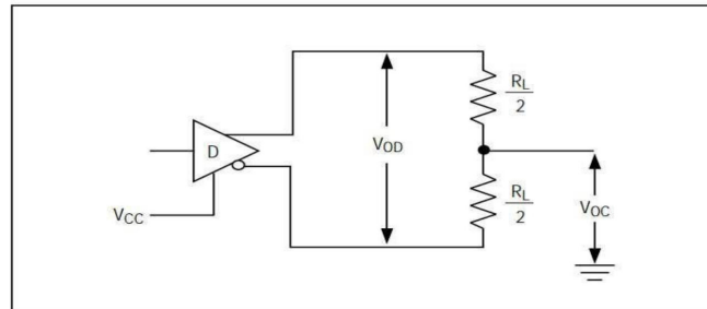
Fig. 2 Driver DC test load
