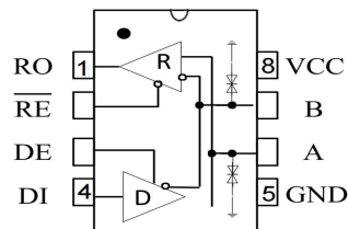
Figure 1 MAX481EESA-TD pin configuration
