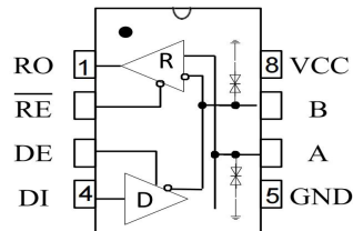
Figure 1 MAX483CSA-TD pin configuration
