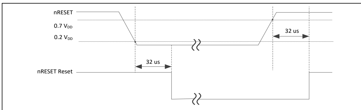
Figure 6.2-3 nRESET Reset Waveform(Except SPDx and DPDx mode)
