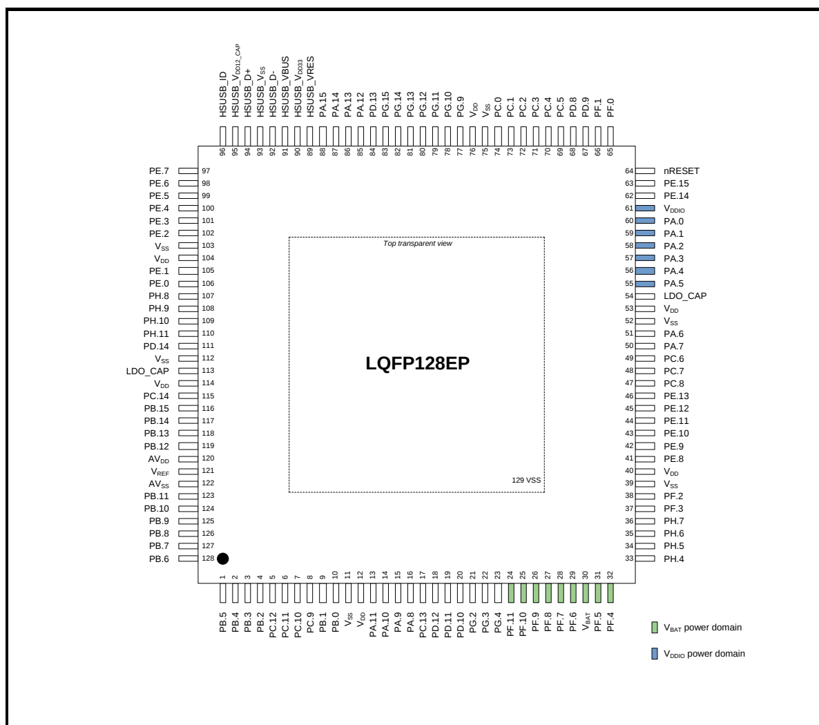
Figure 4.1-7 M463 Series LQFP128 EPAD Pin Diagram
