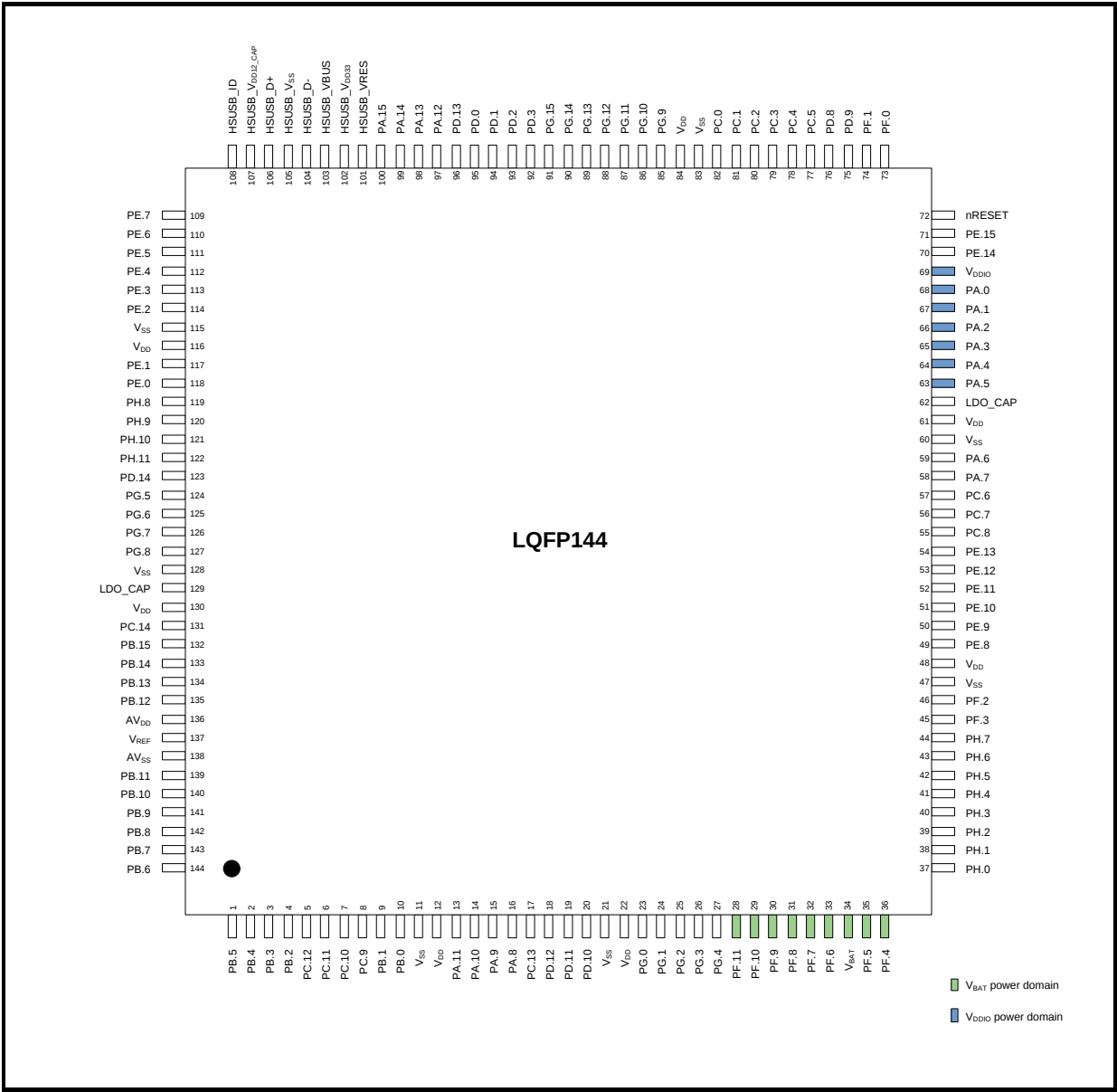
Figure 4.1-10 M467 Series LQFP144-Pin Diagram
