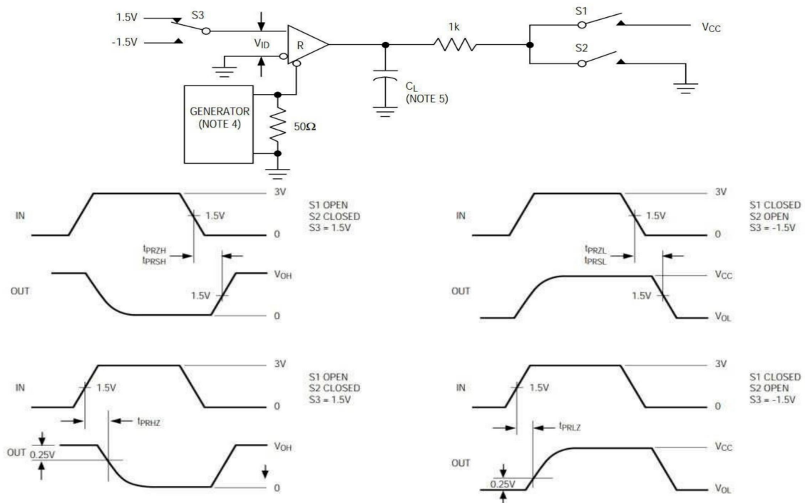
Fig. 8 Receiver enable and disable times
