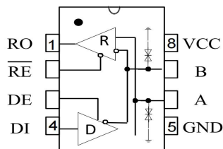
Figure 1 MAX483ECSA-TD pin configuration
