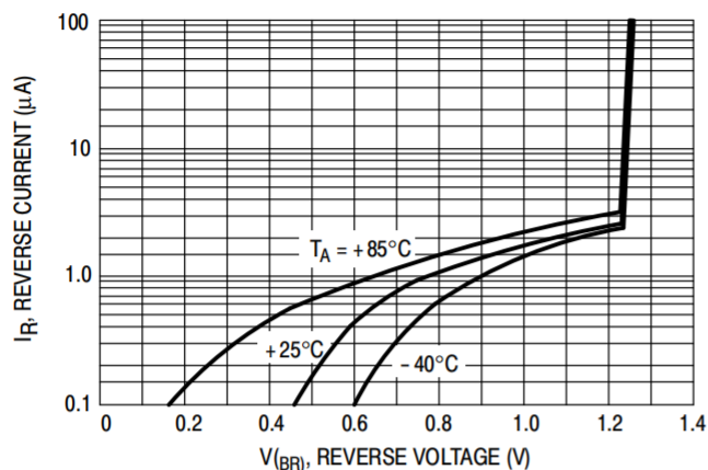
Figure 2. Reverse Characteristics
