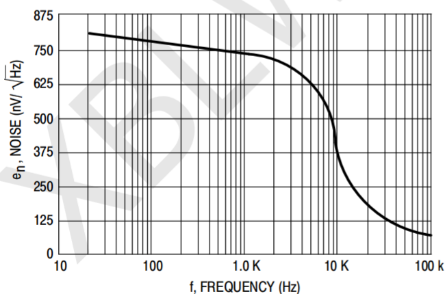
Figure 6. Noise Voltage
