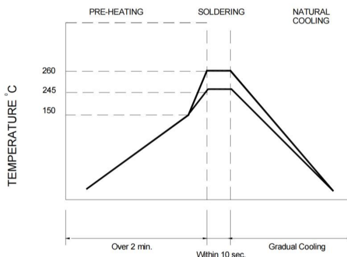
Figure 2. Wave Soldering
