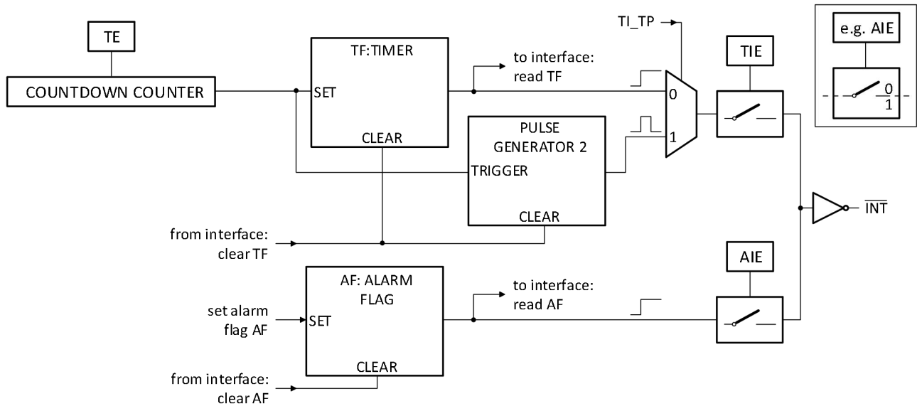
Fig 6. Interrupt scheme
