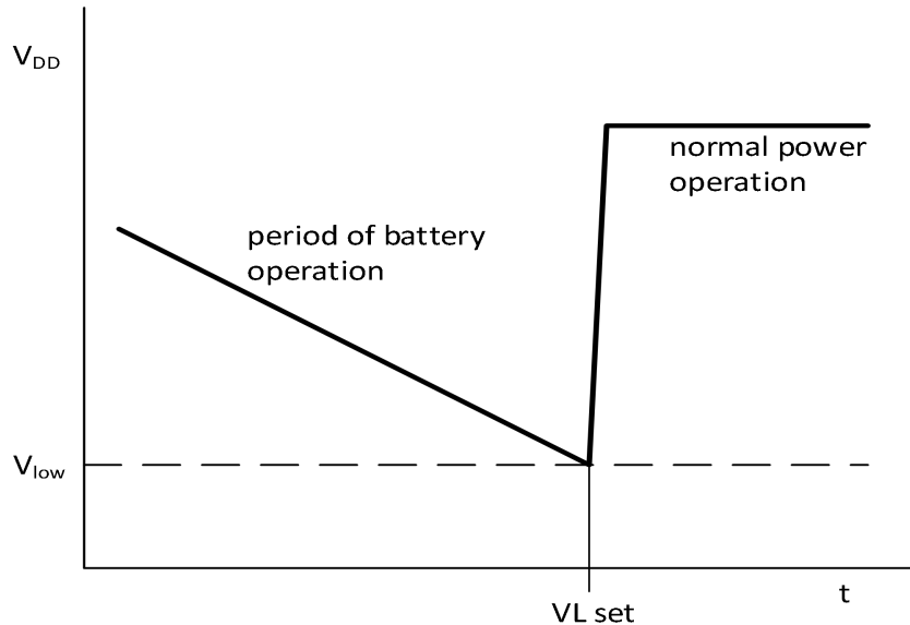
Fig 7. Voltage-low detection
