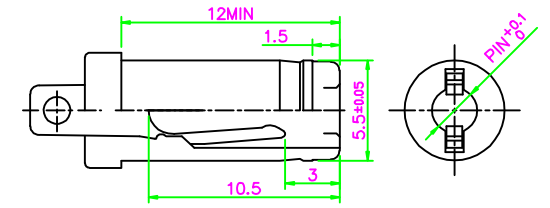
RECOMMENDED PLUG
