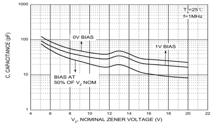
Fig.4 Typical Capacitance
