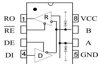
Figure 1 MAX1487CSA-TD pin configuration
