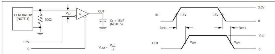
Fig. 7 Receiver propagation delay
