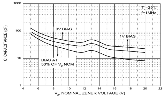
Fig.4 Typical Capacitance
