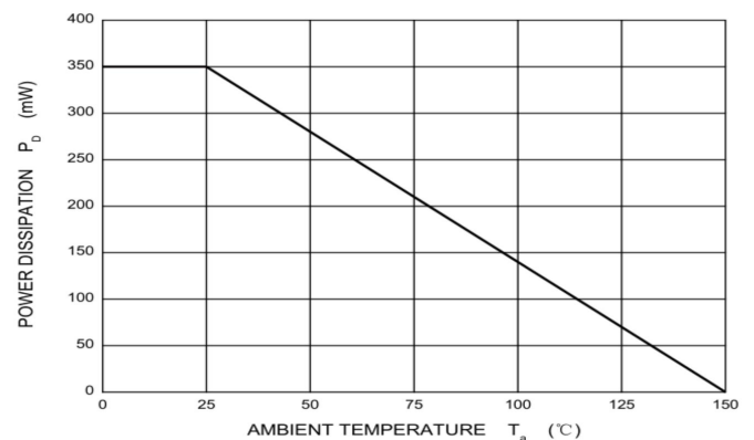
Fig.6 Power Derating Curve
