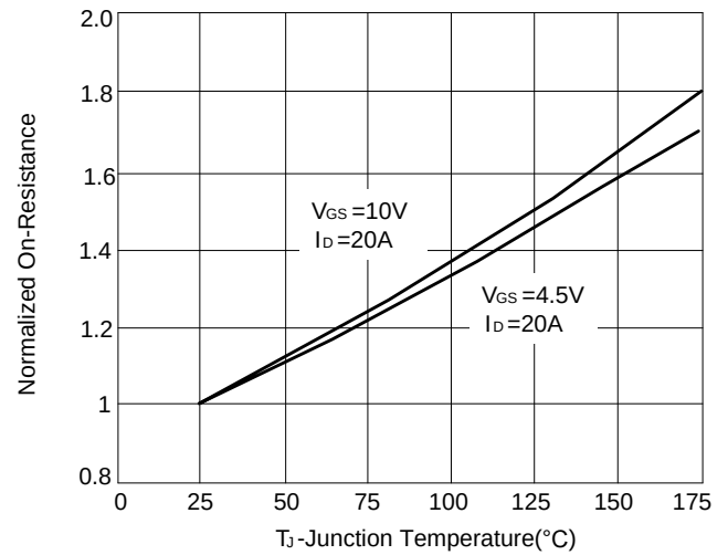
Figure 2: Rdson-Junction Temperature
