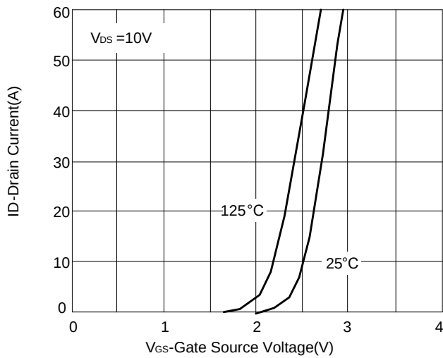
Figure 3: Transfer Characteristics
