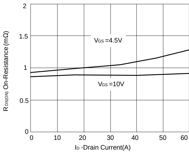
Figure 5: Rdson-Drain Current
