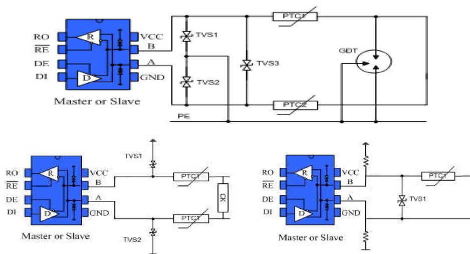
Fig. 11 Port protection scheme
