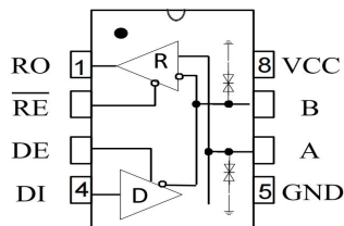
Figure 1 MAX481CSA-TD pin configuration
