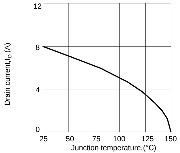
Figure 2: Drain current vs. junction temperature
