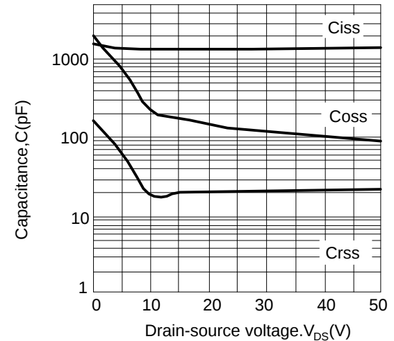
Figure 4: Capacitance characteristics
