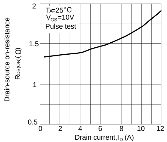
Figure 10: Drain-source on-resistance vs. drain current
