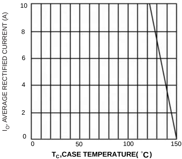
FIGURE.3 Forward Current Derating Curve
