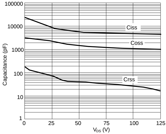
Figure 7: Capacitance Characteristics
