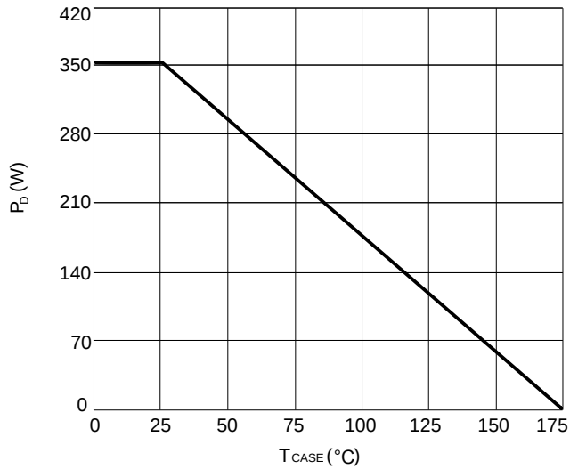
Figure 9: Power De-rating
