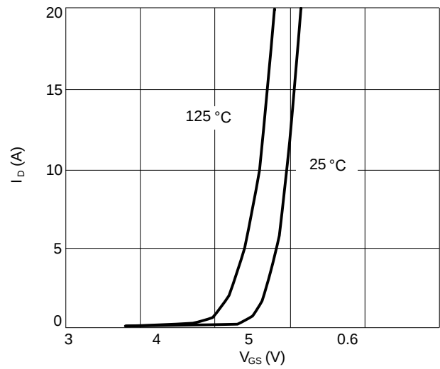
Figure 2: Transfer Characteristics
