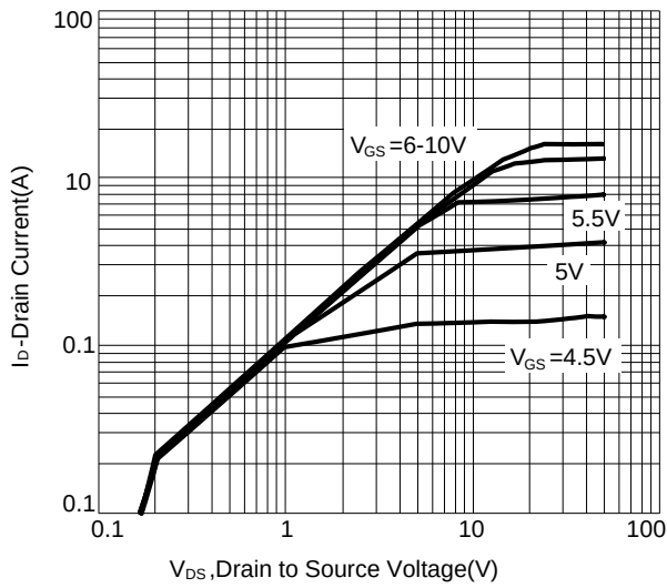
Figure 1: Output Characteristics
