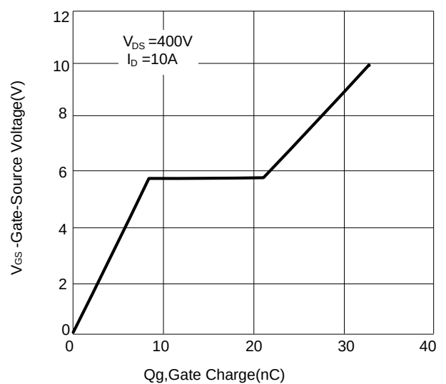
Figure 6: Gate Charge vs. Gate to Source Voltage
