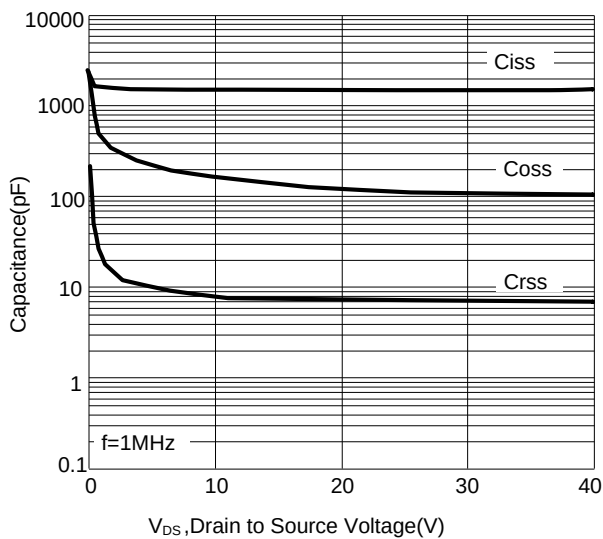
Figure 5: Capacitance vs. Drain to Source Voltage
