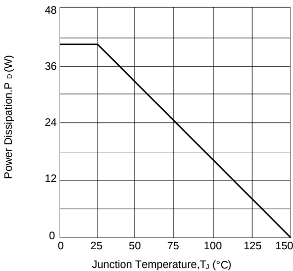
Figure 11: Power Dissipation vs. Junction Temperature
