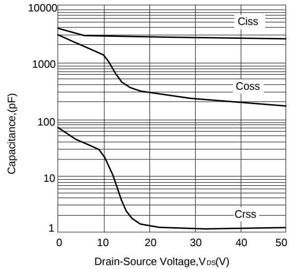
Figure 4: Capacitance Characteristics
