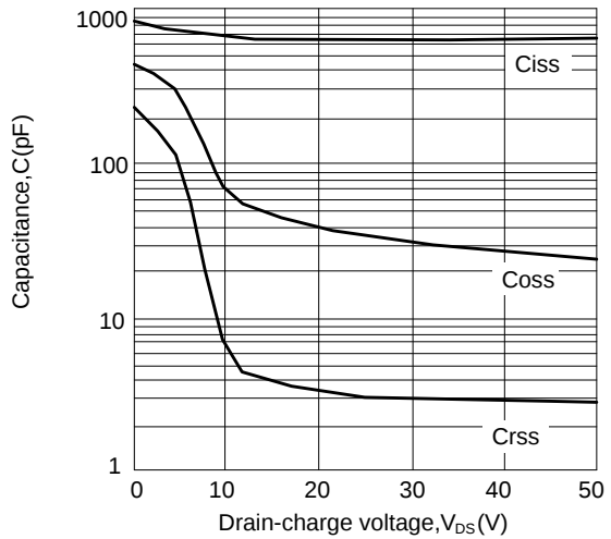
Figure 4: Capacitance characteristics
