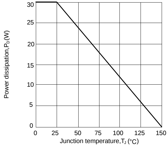
Figure 8: Power dissipation vs. junction temperature
