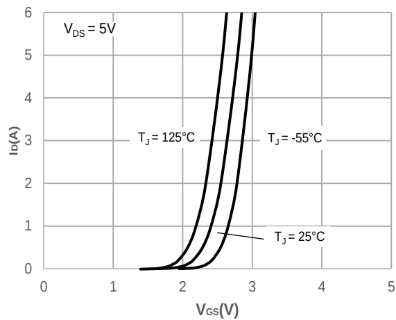
Fig 2. Transfer Characteristics
