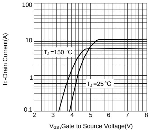
Figure 1: Transfer Characteristics
