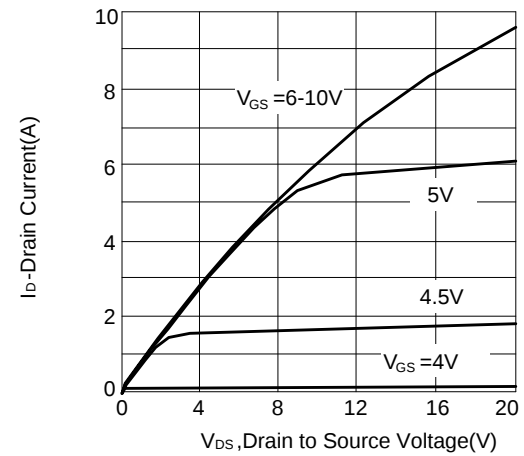
Figure 10: Output characteristics
