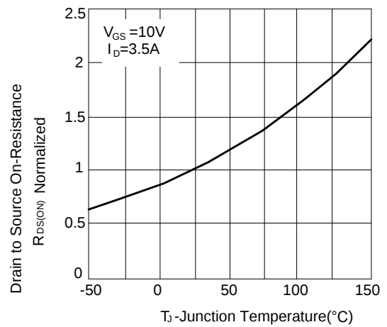
Figure 4: Drain to Source On-Resistance vs. Junction Temperature
