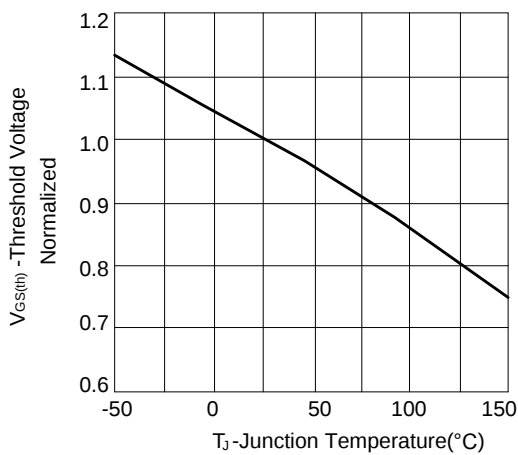
Figure 5: Threshold Voltage vs Junction Temperature
