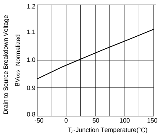
Figure 6: Breakdown Voltage vs Junction Temperature
