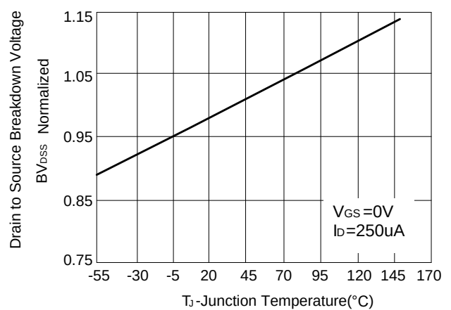
Figure 6: Breakdown Voltage vs Junction Temperature
