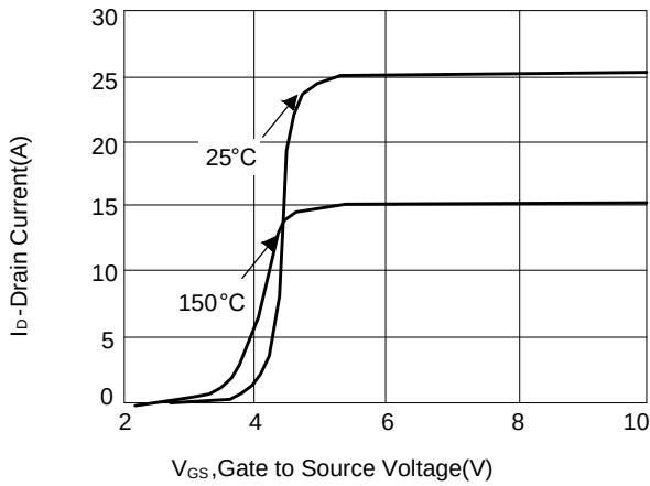
Figure 1: Transfer Characteristics
