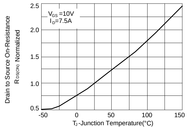
Figure 4: Drain to Source On-Resistance vs Junction Temperature
