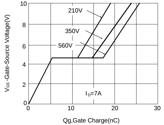
Figure 8: Gate Charge vs Gate to Source Voltage
