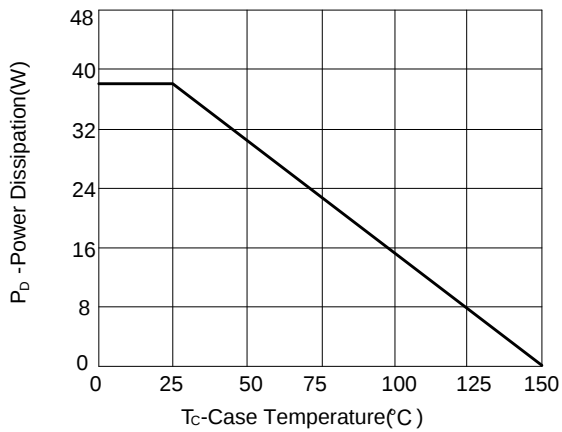
Figure 11: Power Dissipation vs Case Temperature
