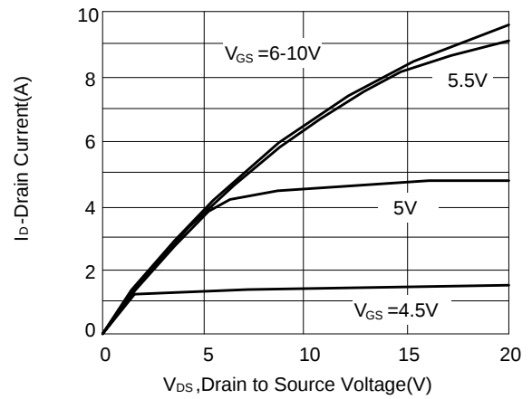
Figure 10: Output Characteristics
