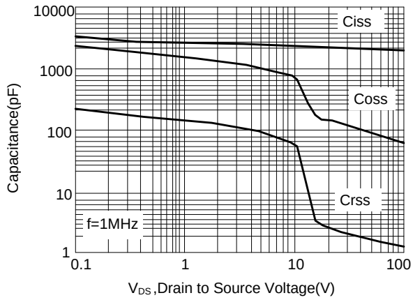
Figure 7: Capacitance vs Drain to Source Voltage
