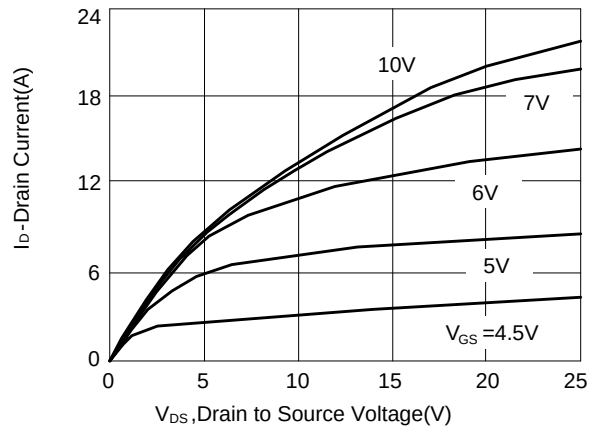
Figure 10: Output Characteristics
