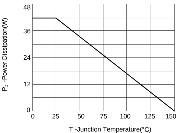
Figure 11: Power Dissipation vs Junction Temperature
