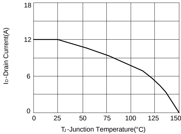
Figure 9: Continuous Drain vs Junction Temperature
