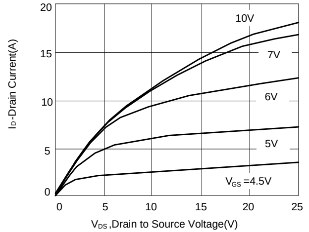
Figure 10: Output Characteristics
