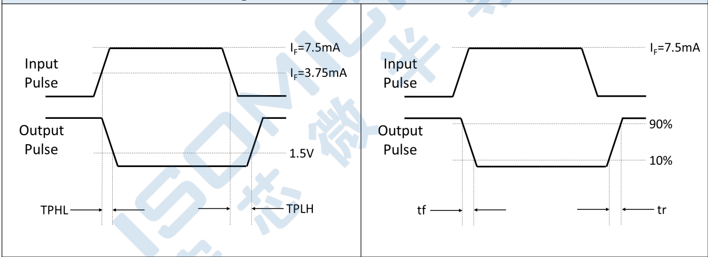
Fig.24 Waveforms of t_{PHL} , t_{PLH} , t_r , t_f
