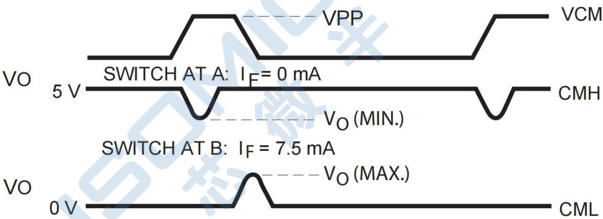
Fig.26 Waveforms of Common Mode Transient Immunity
