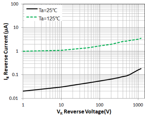
Figure 2. Reverse Characteristic(typ.)
