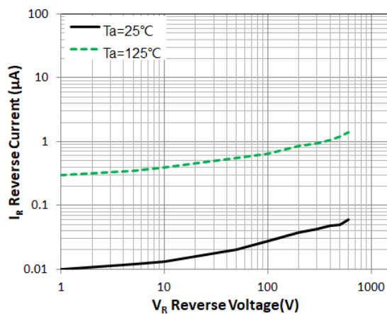
Figure 2. Reverse Characteristic(typ.)
