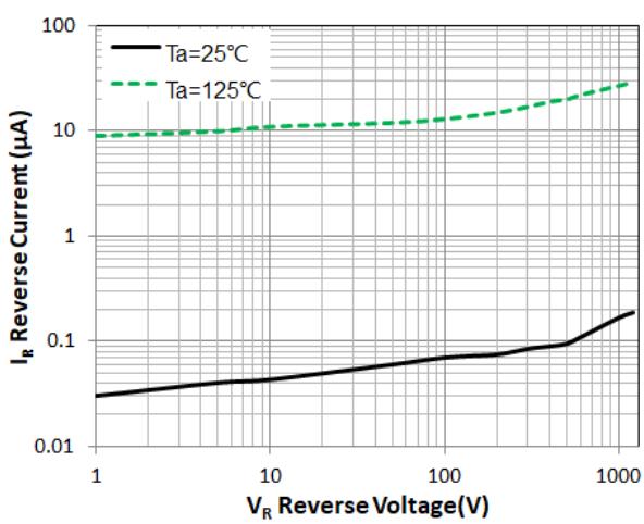
Figure 2. Reverse Characteristic(typ.)
