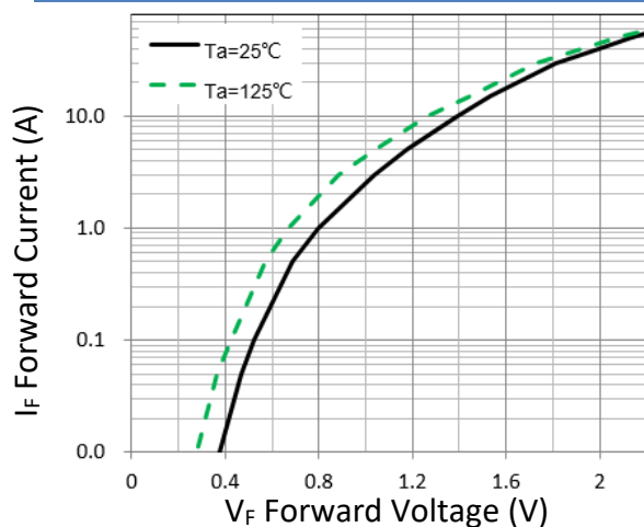
Figure 1. Forward Characteristic(typ.)
